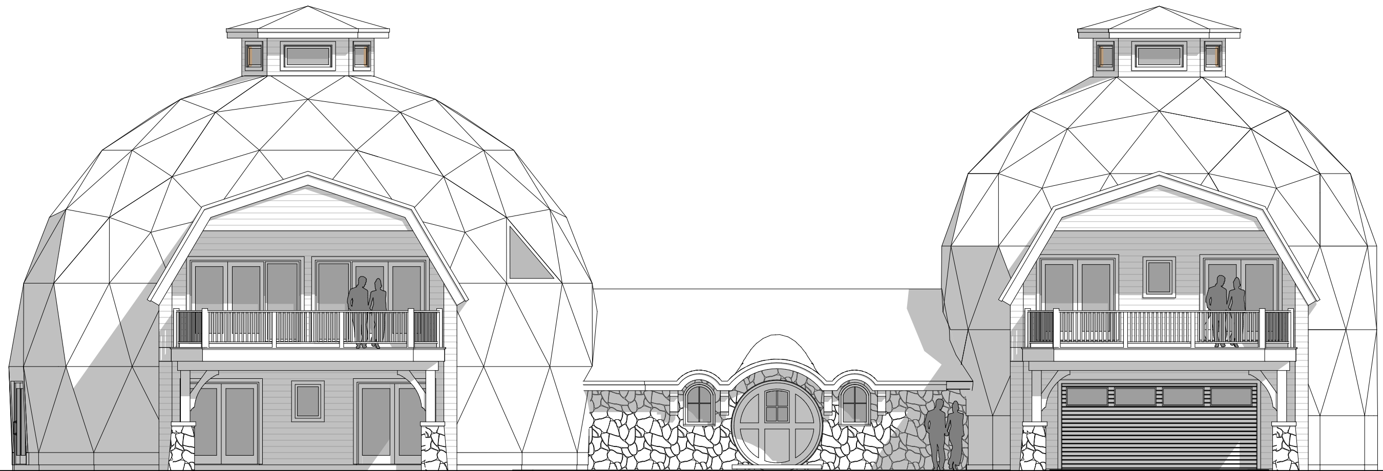
NORTH ELEVATION
