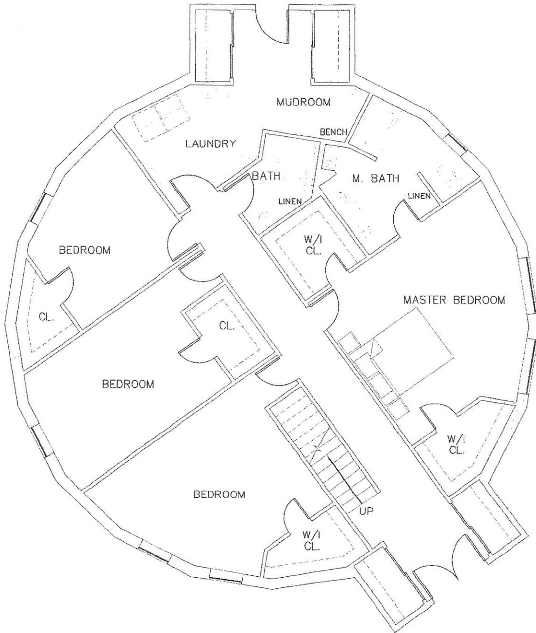
MAIN LEVEL PLAN 8-009
