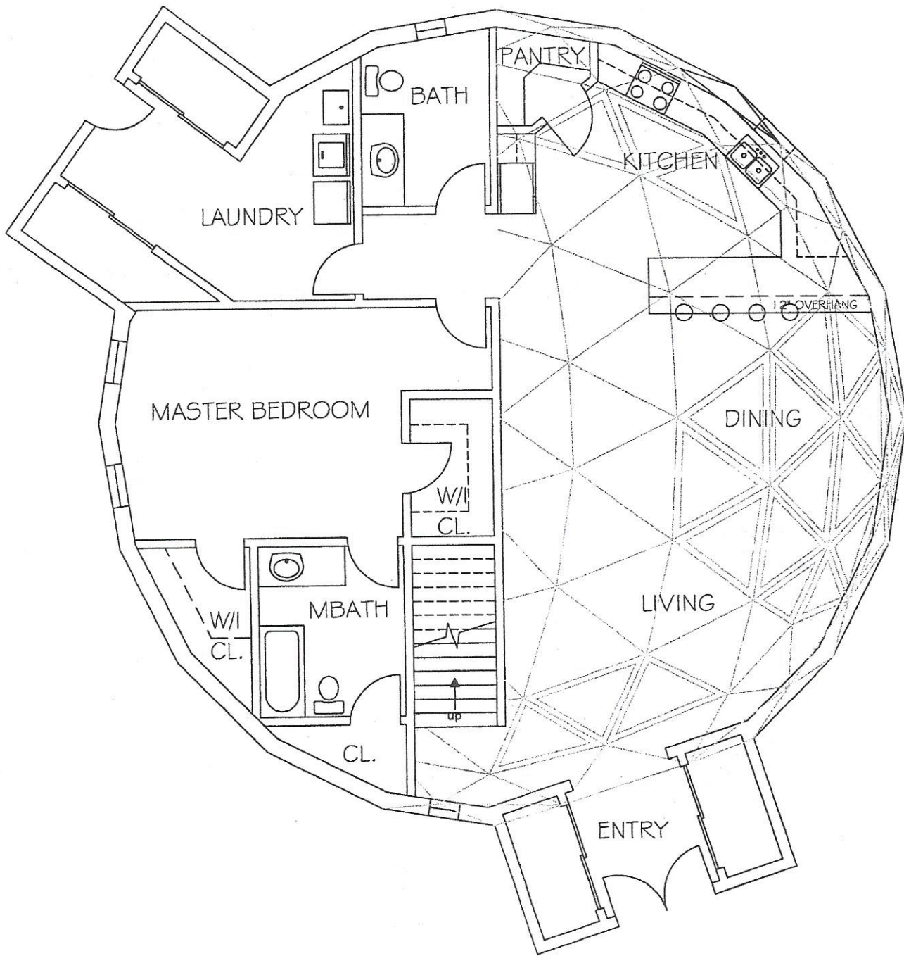
Main Level Plan
