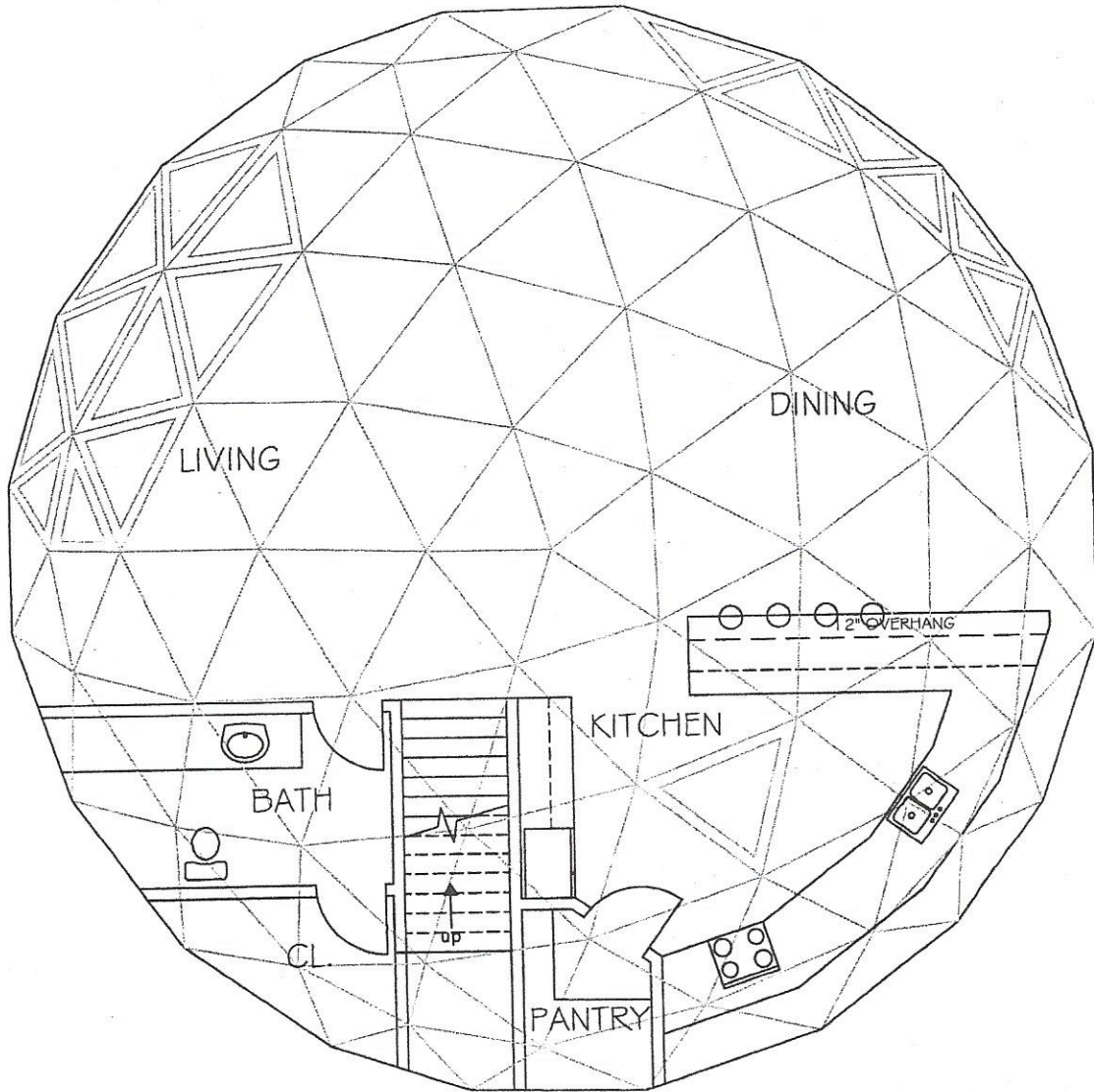
Upper Level Plan
